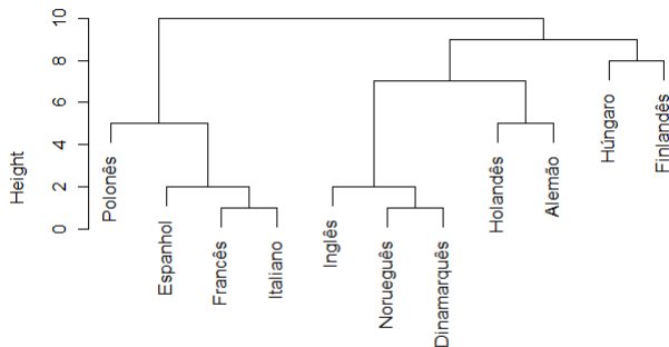
Cluster Dendrogram
